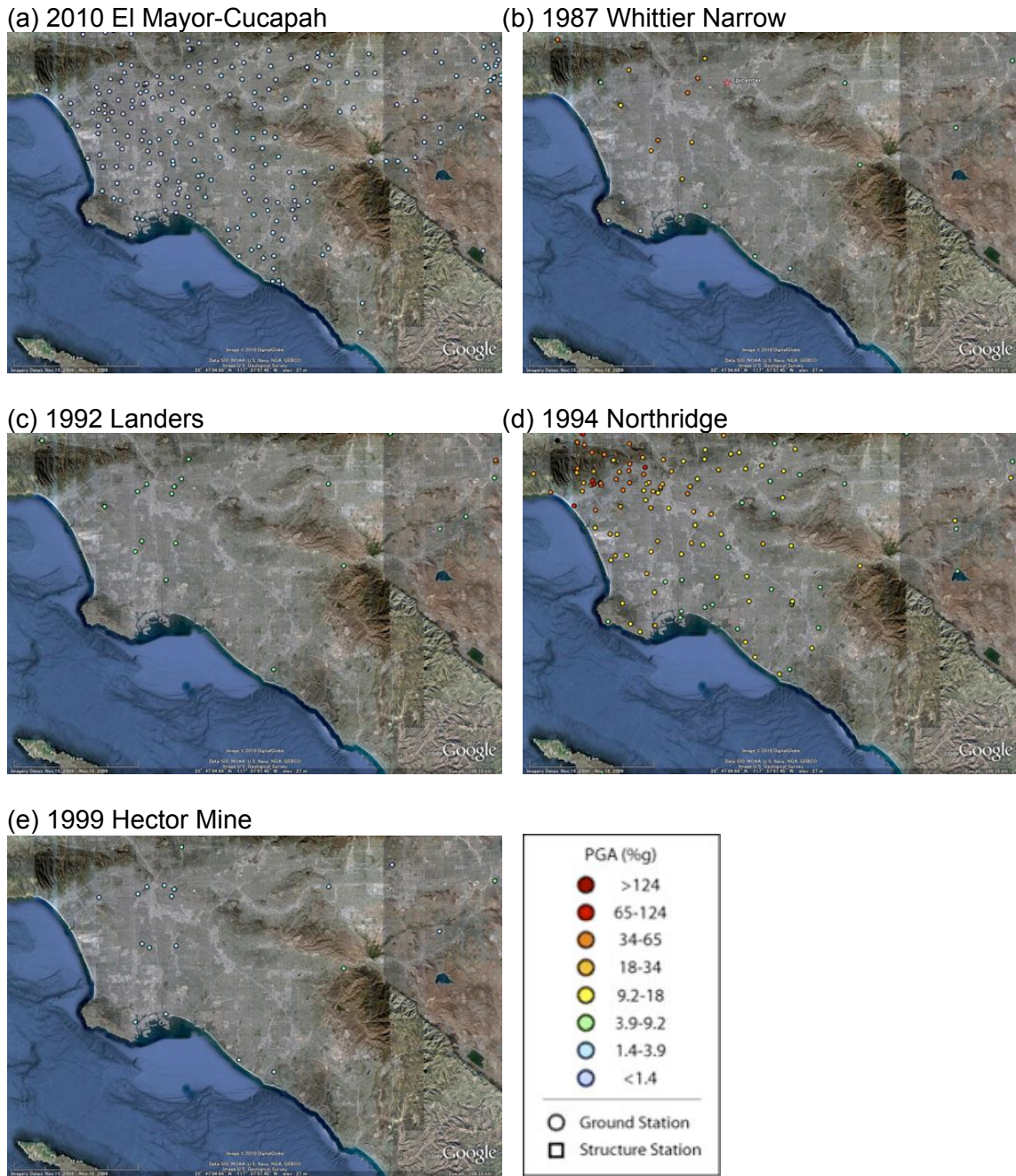
Fig. 2. Significant earthquakes in southern California since 1987, and recorded peak-ground accelerations (PGA); the 2010 El-Mayor Cucapah earthquake has the largest number of recordings.
