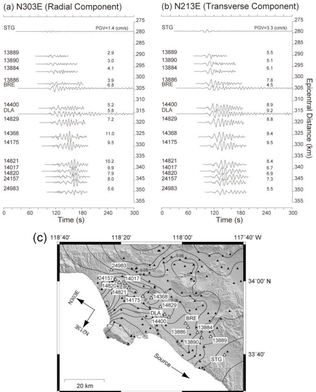
Fig. 5. Velocity waveforms in the LA basin. (a) N303°E-, (b) N213°E-component, (c) The stations whose records are plotted in (a) and (b) (white triangles), along with the same PGV contours (solid lines) and the same stations (black triangles) as shown in Figure 4. The N303°E and N213°E correspond to the radial and transverse directions, respectively, with respect to the one from the source to the basin. The waveforms were bandpass-filtered with a passing period range of 3 to 16 s.
